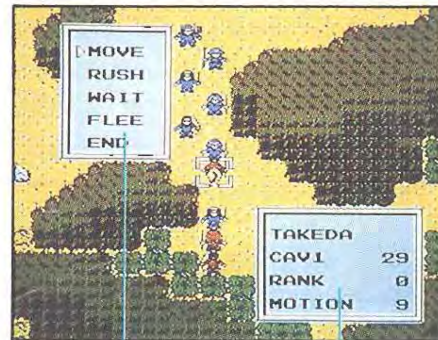
Command Window
